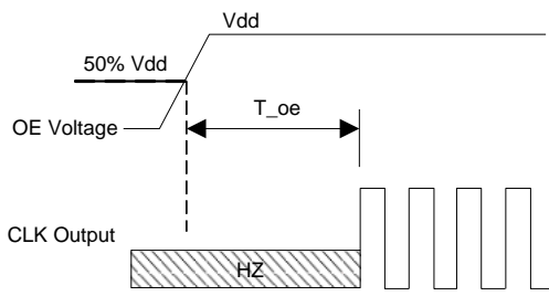
Figure 6. OE Enable Timing (OE Mode Only)
