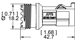
Male Receptacle SK1-019M03
